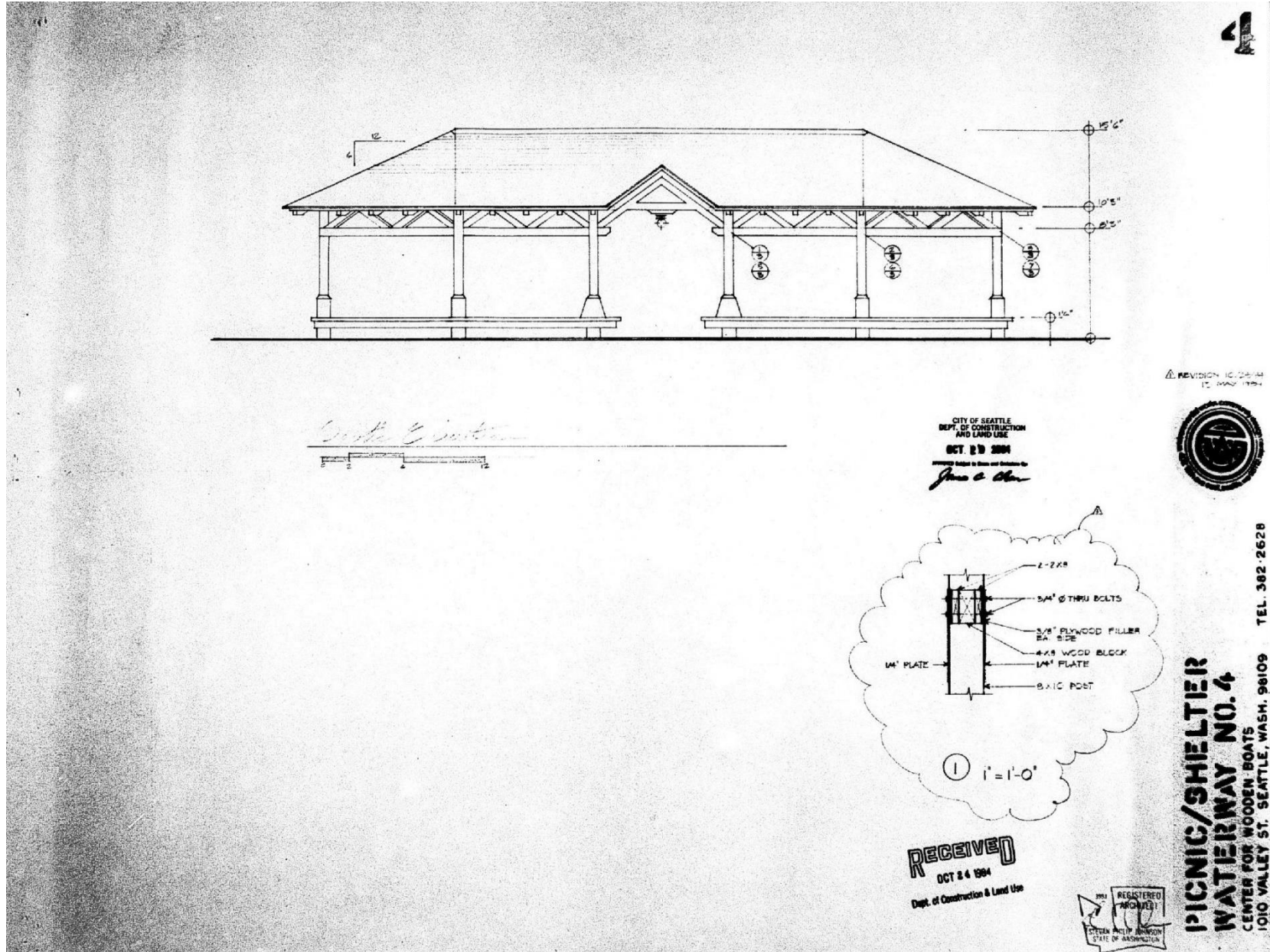
D9. Pavilion Project: Elevation drawing, Center for Wooden Boats, 1984. Source: City of Seattle, Dept. Construction & Inspections.
