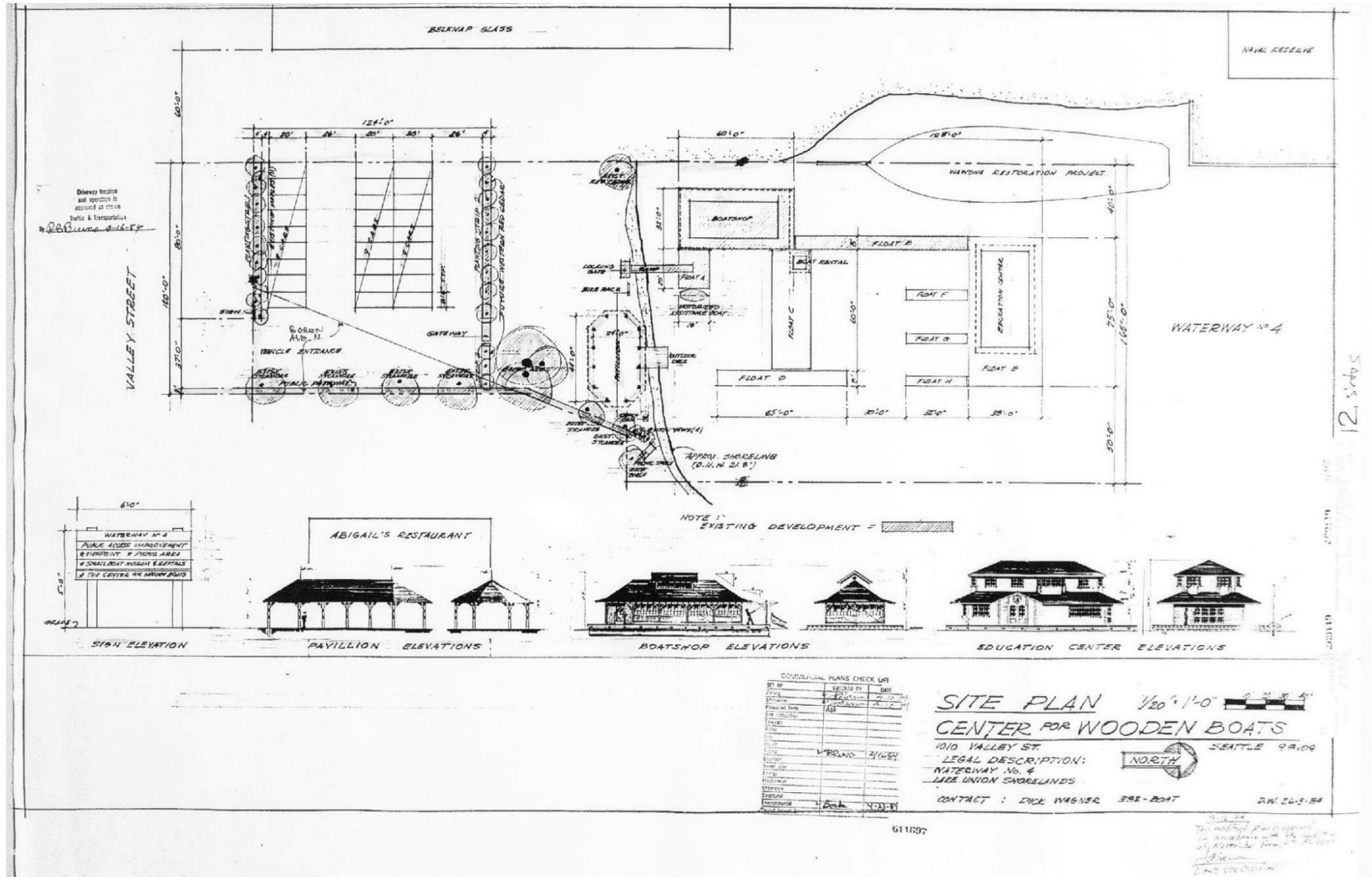
D5. Site plan, Center for Wooden Boats, Dick Wagner, 1984. Source: City of Seattle, Dept. Construction & Inspections.
