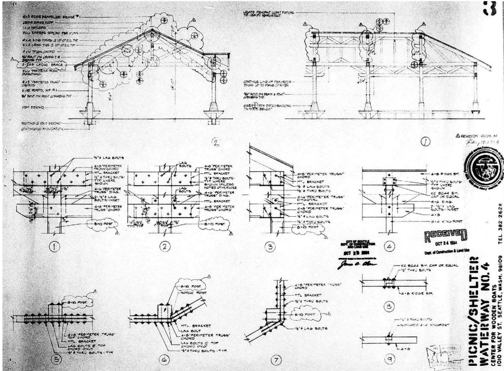
D8. Pavilion Project: Detail drawings, Center for Wooden Boats, 1984. Source: City of Seattle, Dept. Construction & Inspections.
